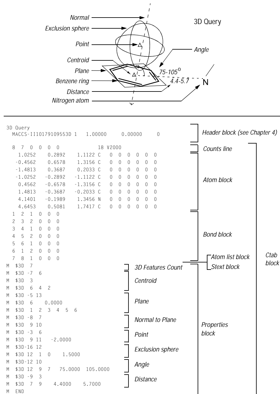
Figure 7 Ctab organization of a 3D query
