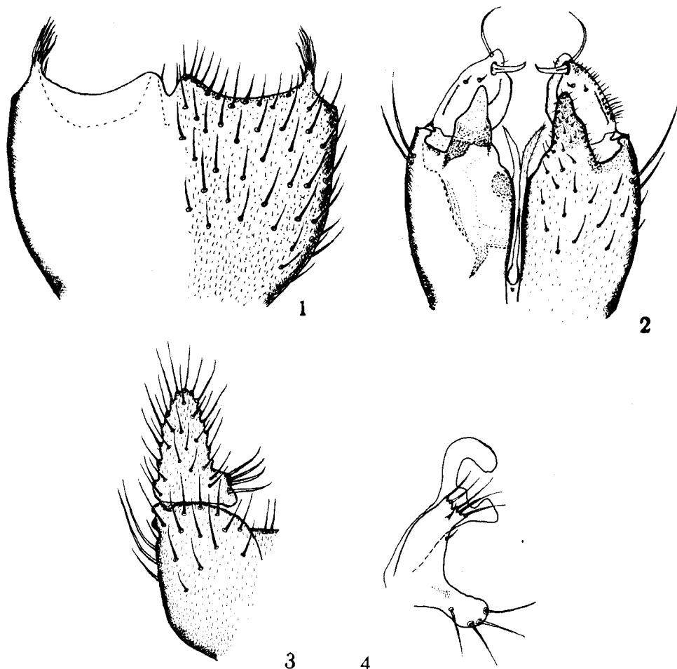
Figs. 1–2: Ectrepesthoneura ledenikiensis n. sp.: 1 – tergite IX; 2 – hypopygium, ventral view. – Figs. 3–4: Mycetophila devioides n. sp.: 3 – Hypopygium, half, ventral view; 4 – dorsal stylomere (dististyle).
